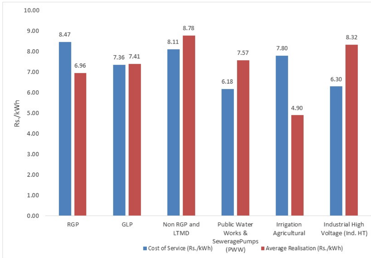
Figure 2: Category-wise cost of service and average realisation of MGVCL (Rs./kWh)
